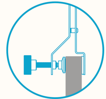
Thickest compatible whiteboard: 25 mm
