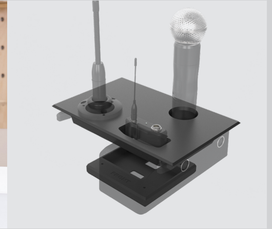
H919 Console Insert for Shure SBC 220 and Gooseneck
