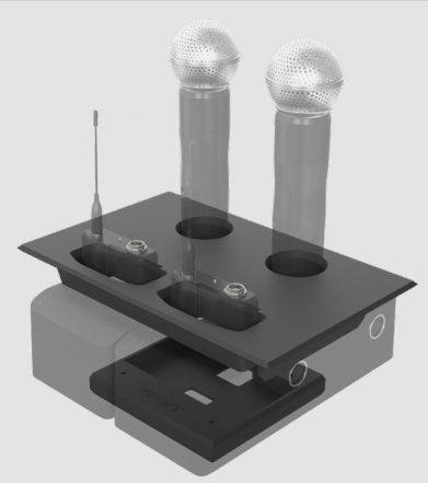
H911 Console Insert for Dual Shure SBC 220 or SBC 240
